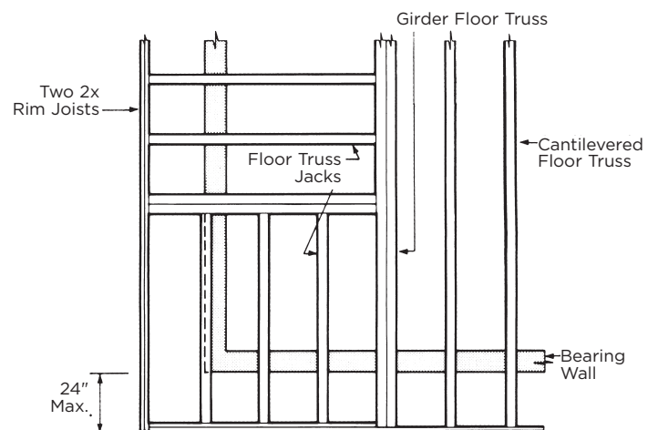
Floor Cantilevered Parallel to Floor Truss Span
