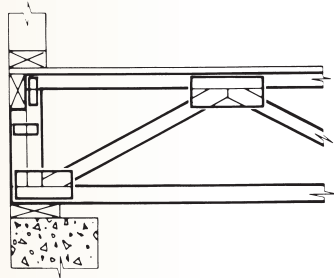
Bottom Chord Bearing on Exterior Frame or Masonry Wall
