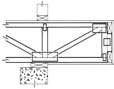
Balcony Cantilever Special Engineering Required
