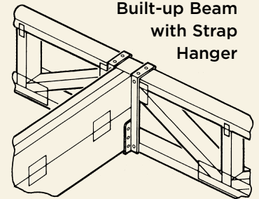
Header Beam Pocket
