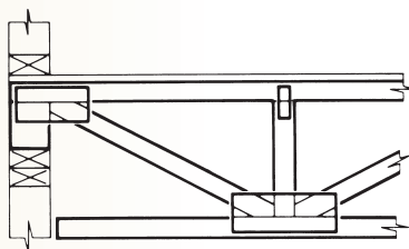
Top Chord Bearing on Frame Wall
